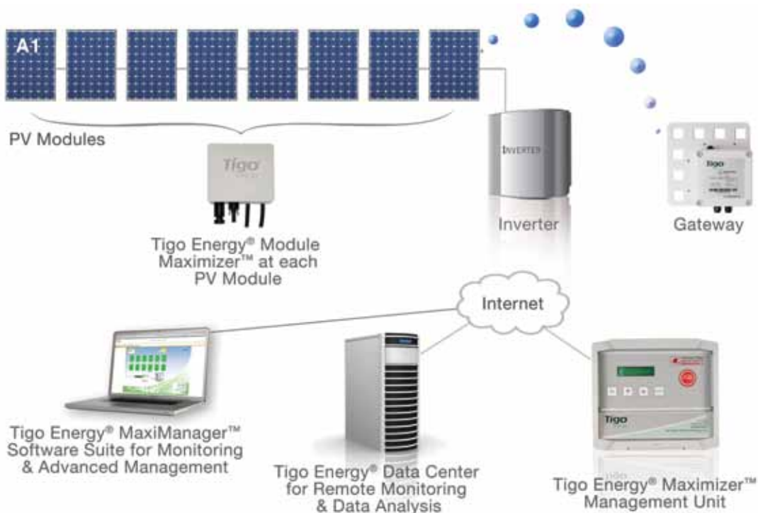
Figure 6 - Tigo Energy system configuration
