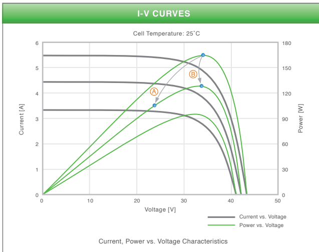
Figure 9 I-V & Power Curves
