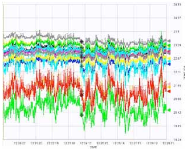
Figure 2 – Voltage distribution of a typical crystalline PV string (Berkeley, CA - 2008)
