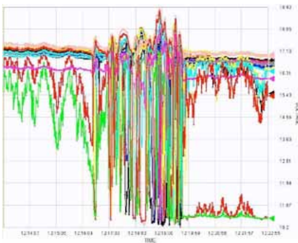
Figure 3 – System impact of a cloud (Santa Cruz, CA)
