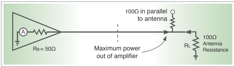
Figure 5b - RF impedance matching
